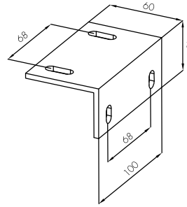
Laibungswinkel XL support for reveal mounting
