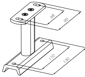
Distanzkonsole U-XL distance bracket U-XL
